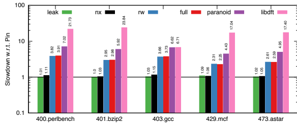
Figure 1: Performance impact of user-provided mitigations.
