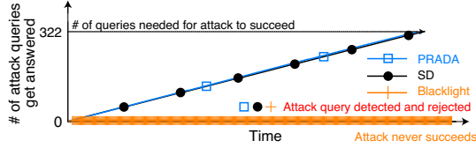
Figure 7: By detecting/rejecting most of attack queries (regardless of account usage), Blacklight effectively resists persistent attackers, which existing defenses fail to address.
